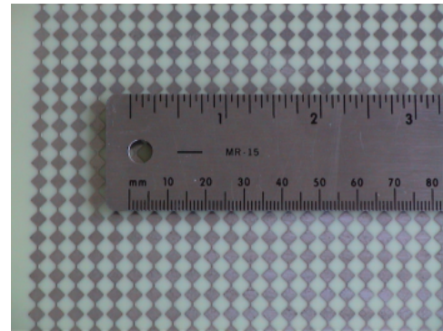
Figure 6: Part of the prototype's antenna array. Compare with Figure 5.
